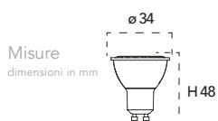
Lampadina a Led 4W, 240V
