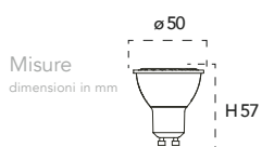
Lampadina a Led 6W, 240V KIT 20
