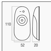
KIT CONTROLLER RGB+W + TOUCH REMOTE
