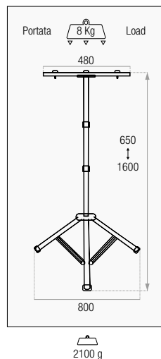
TREPIEDI / TRIPOD
